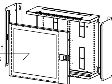
Exploded view
