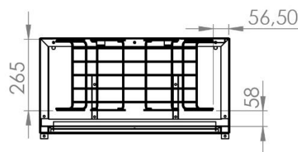
TOP INSIDE VIEW
