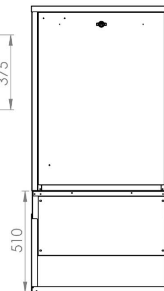
FRONT MAX VIEW
