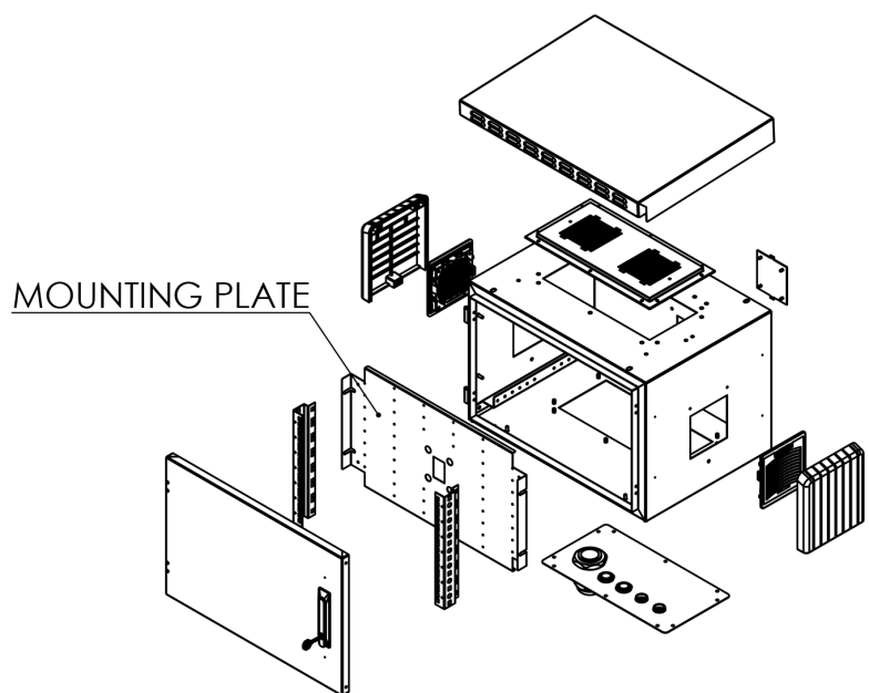
EXPLODED VIEW
