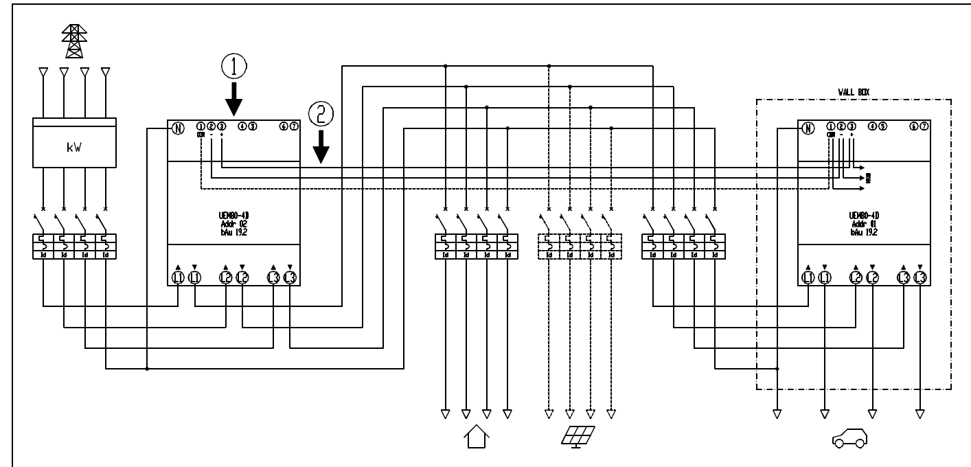
TYPICAL INSTALLATION EXAMPLE
