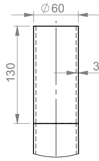
DETAIL A SCALE 1 : 5
