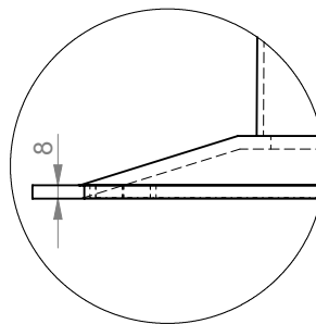
DETAIL D SCALE 1 : 5
