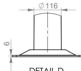
DETAIL D SCALE 1 : 10
