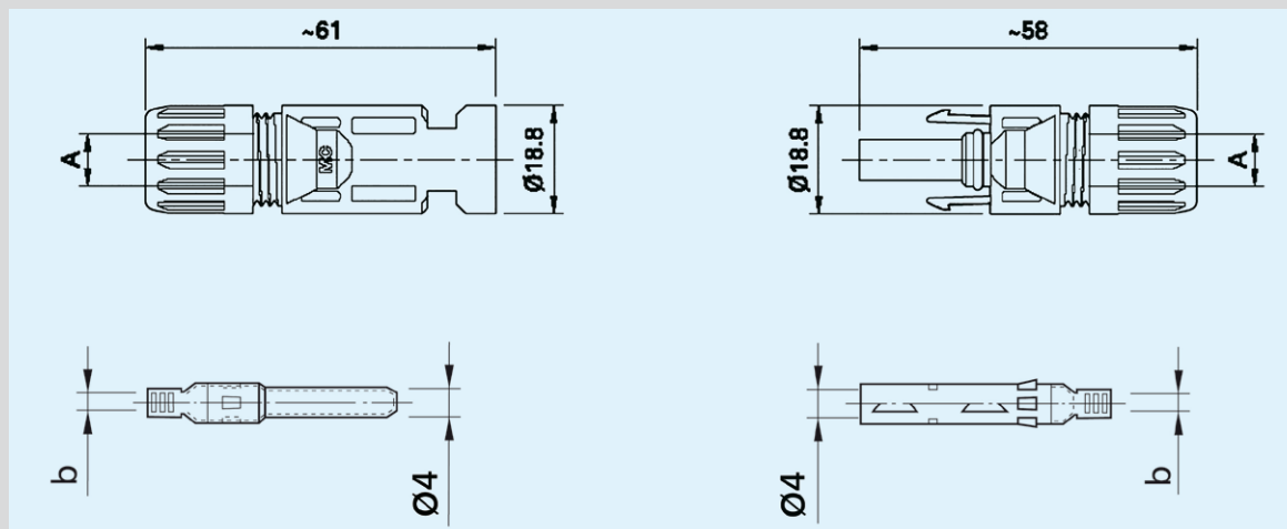
PV coupler plug PV-KST4 ...
