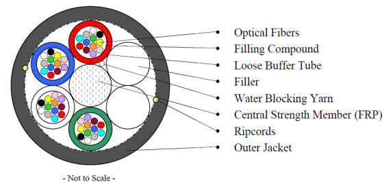
Ex 48 fiber cable
