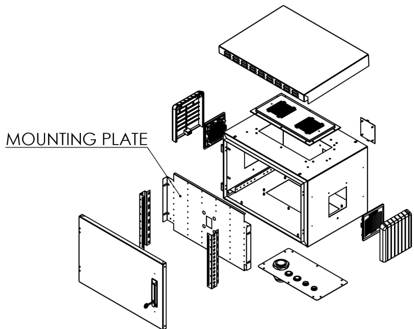
EXPLODED VIEW
