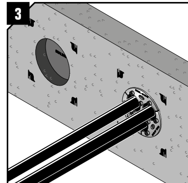
Insert the Roxtec seal.
