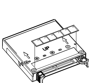
Copper Cassette
