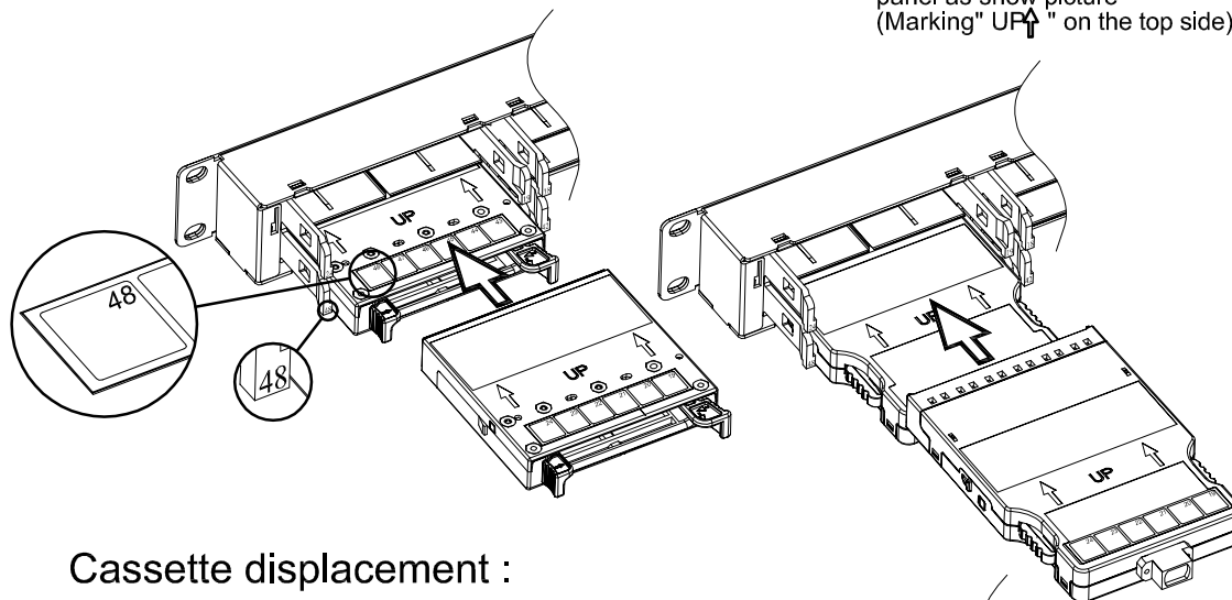
Copper Cassette
