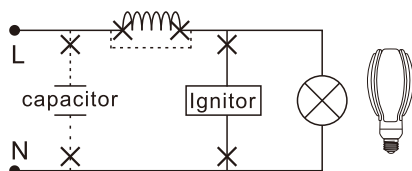
LED Olive Bulb Wiring Diagram
