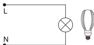
LED Olive Bulb Wiring Diagram
