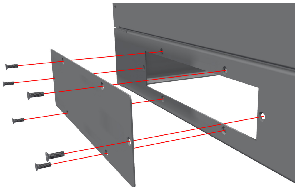
Figure 3.1 Plinth covers
