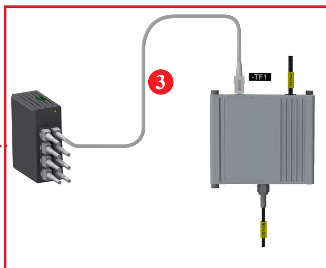
Figure 4.11 Connecting the 4G router
