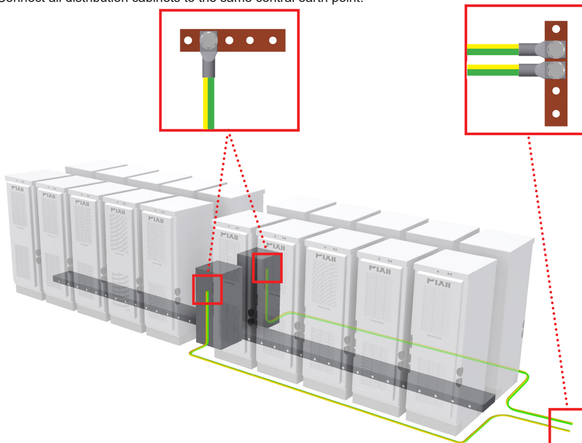
Figure 4.3 Distribution cabinets bonding
