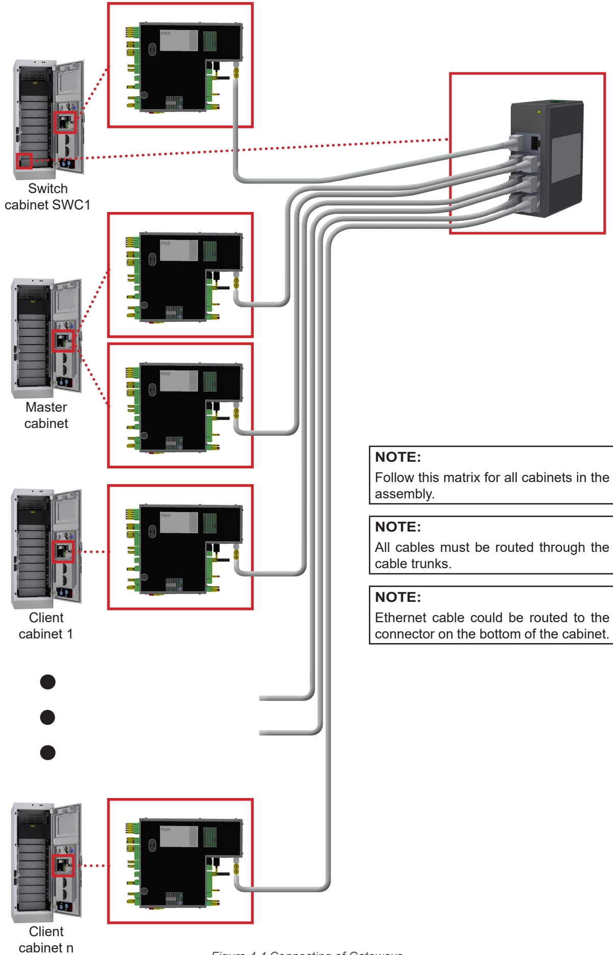
Figure 4.4 Connecting of Gateways
