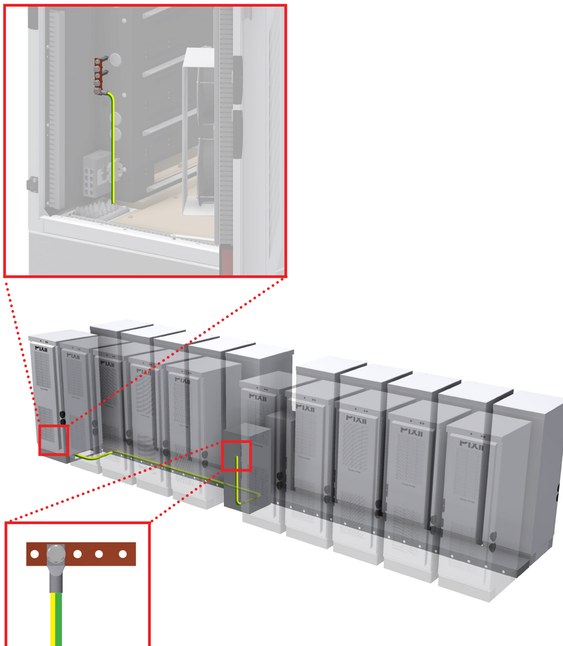
Figure 4.1 Cabinets protective bonding
