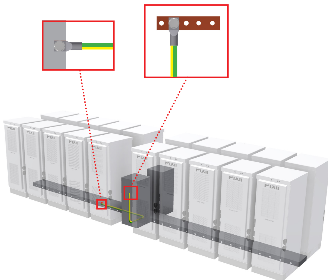
Figure 4.2 Cable trunks bonding
