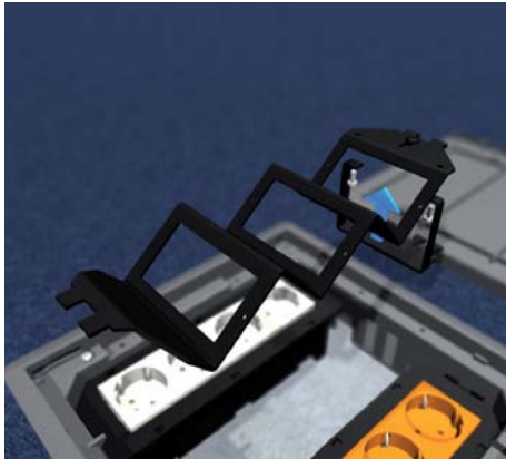
1 | Strain relief Screw device carrier with strain relief tight before installation.
