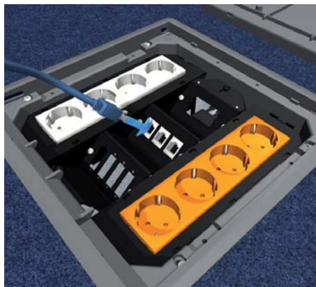
5 | Tailoring Complete device cup with the corresponding cables of manufacturer. Note the installation height.
