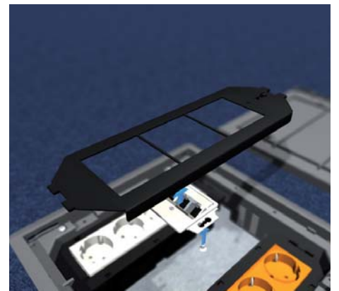
6 | Device carrier Insert installation devices with couler clip into the device carrier from below and screw tight. Insert cover from above.
