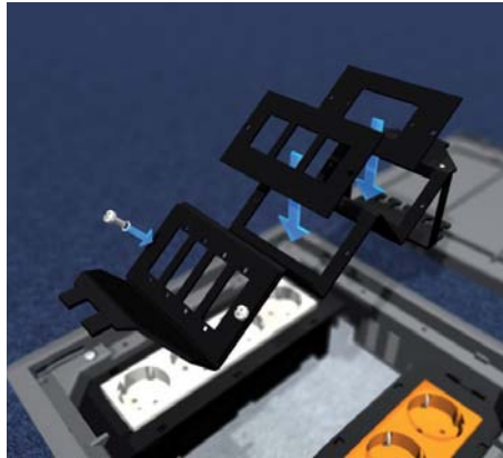
2 | Fitted board Equip device carrier with up to three fitted boards according to the product specifications and screw tight.
