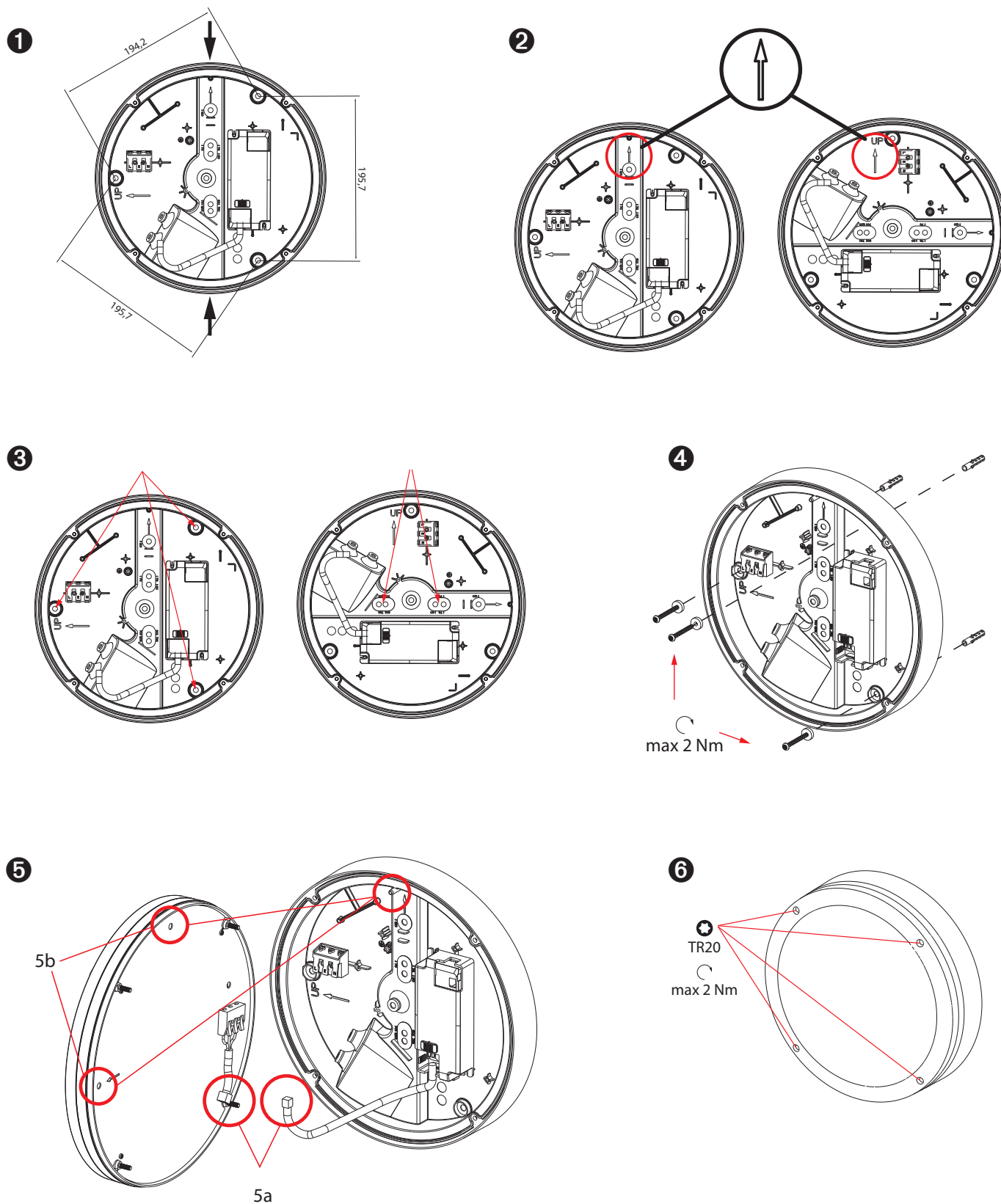
5a Connection of LEDs / 5b Position of diffuser
