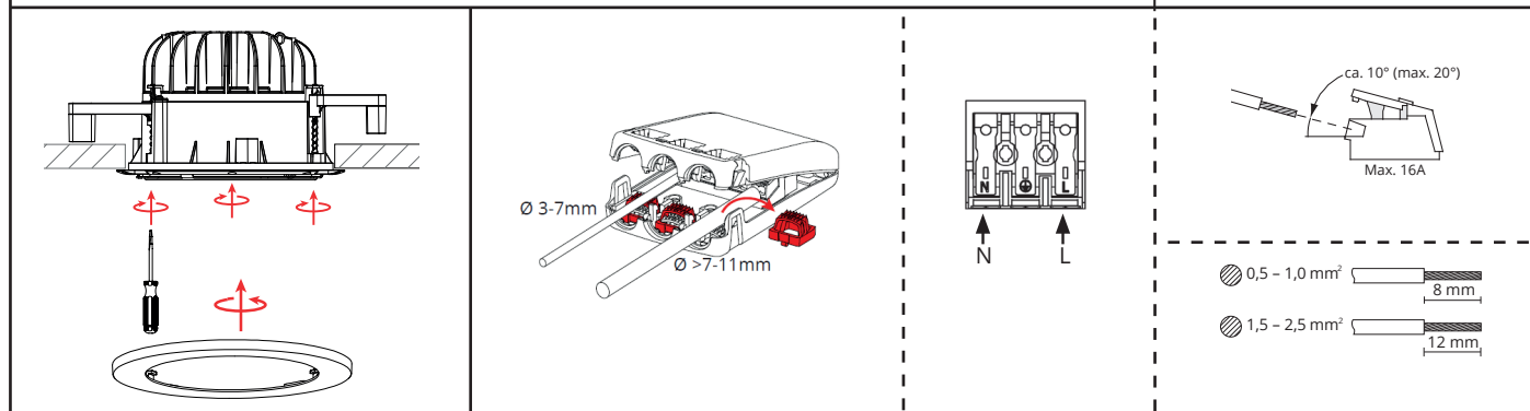
TW LEDDim Smart SG Article number: 820384
