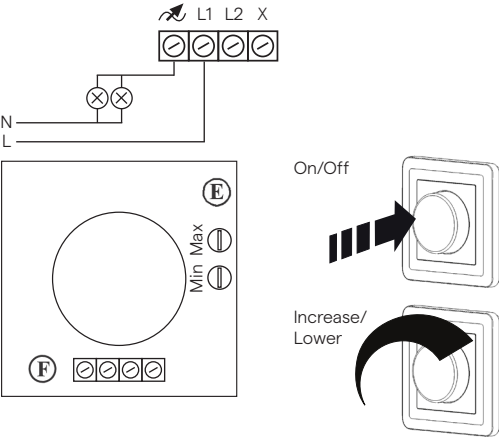
Connection drawing
