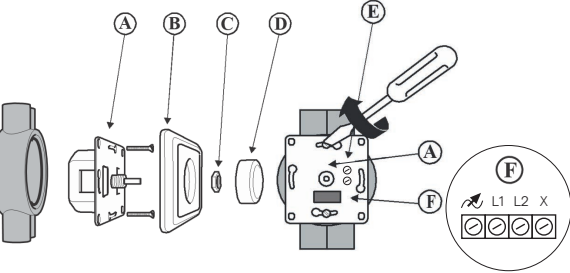
Connection drawing
