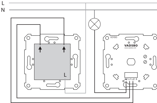
Connection drawing
