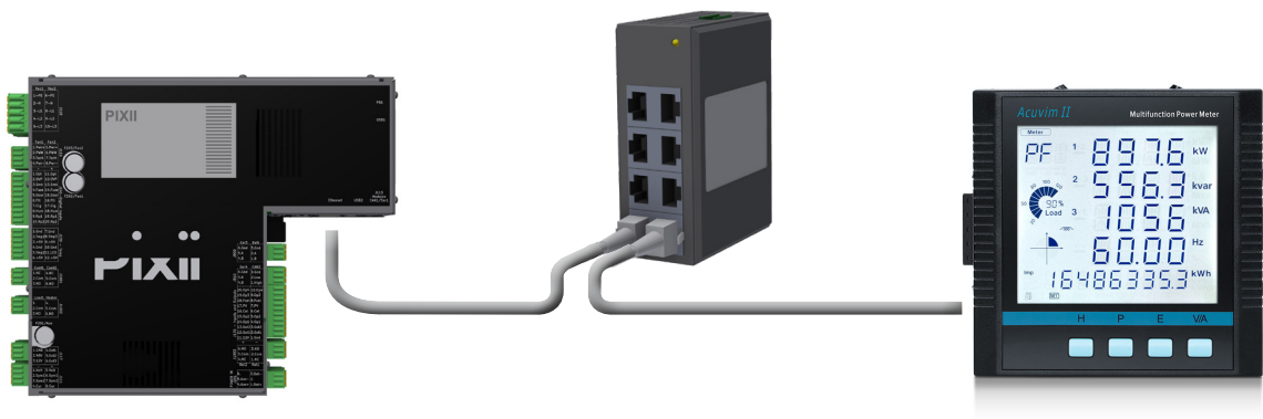
Figure 4.11 Modbus/TCP connection
