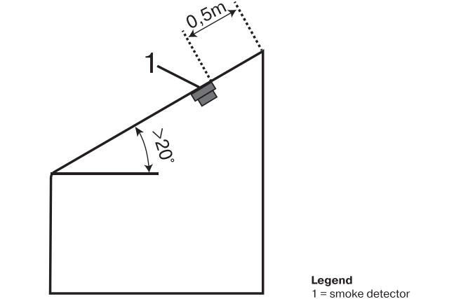
Example of mounting with pedestal-shaped ceiling with a ceiling slope > 20°
