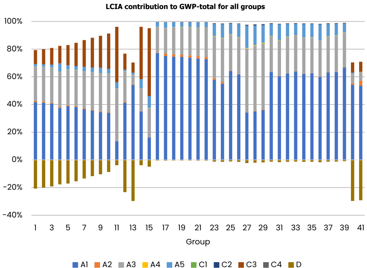
Figure 8– LCIA contribution to GWP total for all groups.
