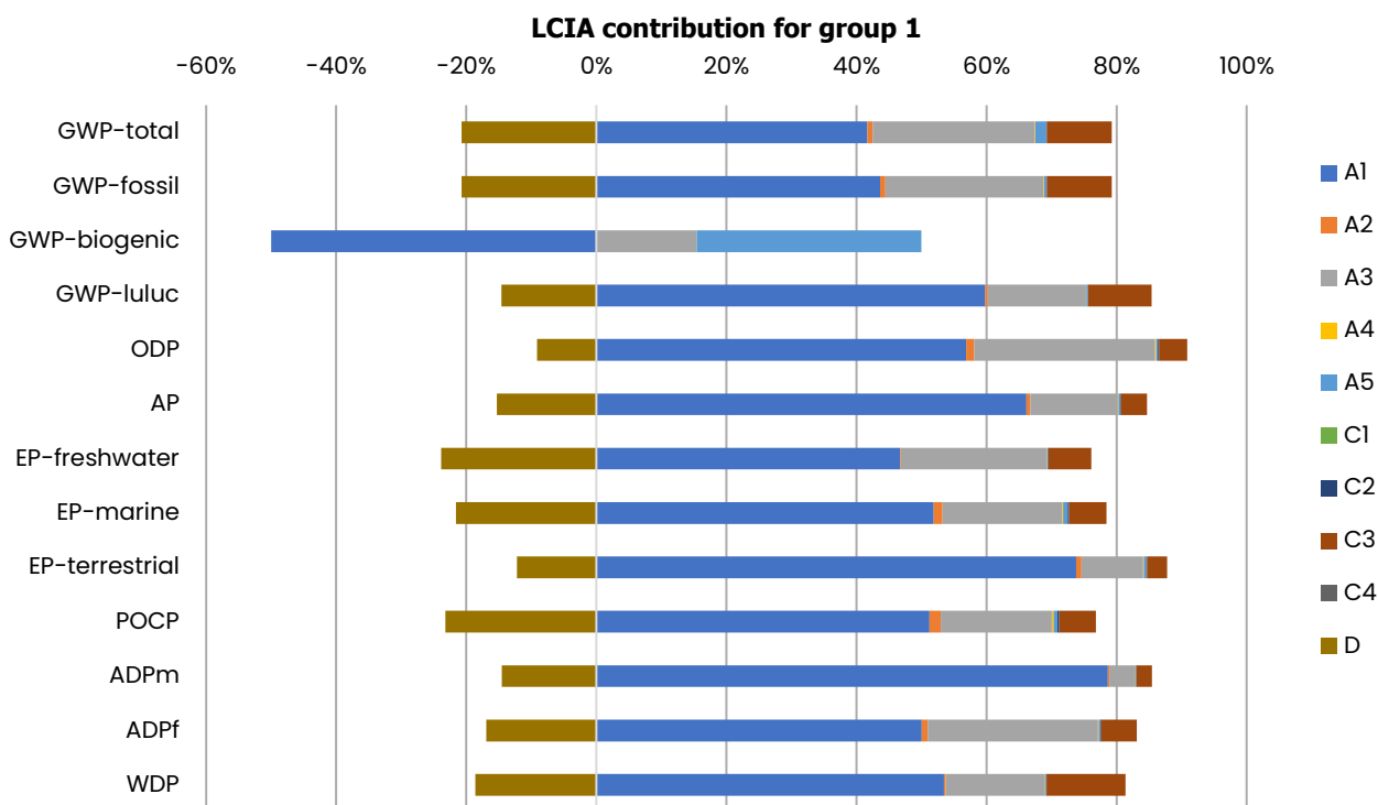
Figure 7– LCIA contribution for group 1.
