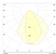
20W Asymmetrisk
