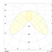
20W Bi-symmetrisk
