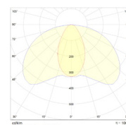
36W Bi-symmetrisk
